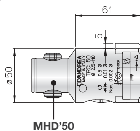
MHD'50
